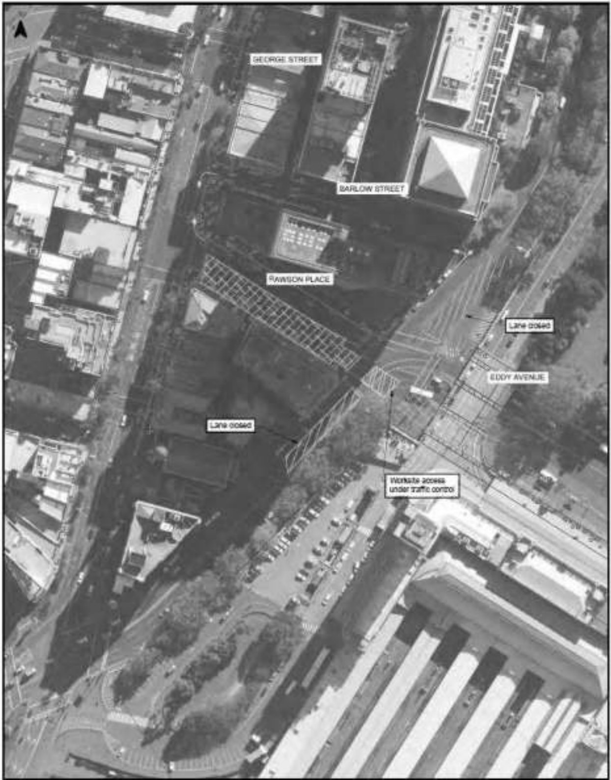
Rawson Place - Stage 2 Intersection Works CSELR Scale: LPM8.2011 0 25 50 100 FT APR 2012 6/2/2012
