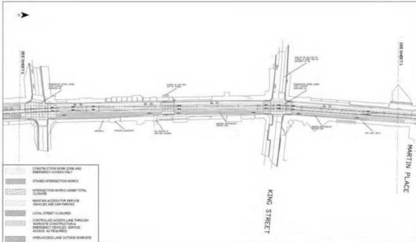
CSELR Local Access - CBD Construction Zone 4 Source: UPM 0211 AUG 2015 10/20/15 0 50 100 200 Feet
