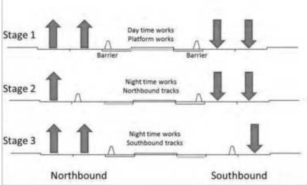
Figure 4-41: Constrained Road Width Construction Staging
