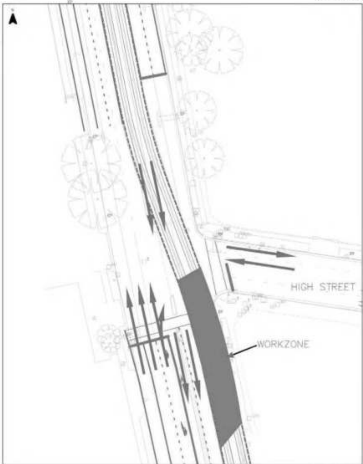
CSELR JUN 2012 HIGH STREET INTERSECTION STAGE 2 Source: LPWA 2011
