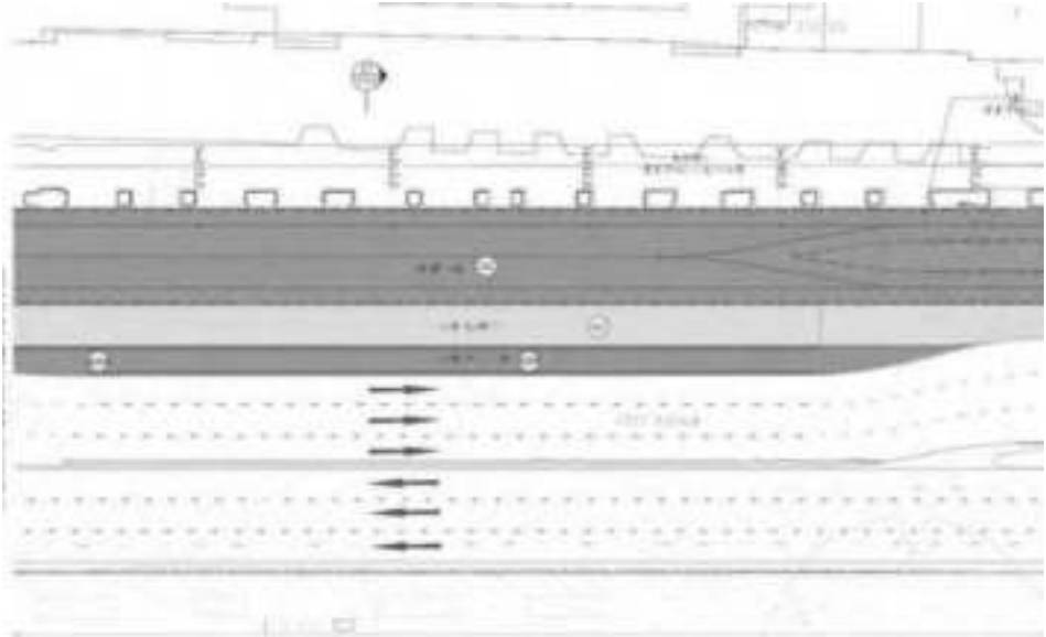
Figure 5-5: Light rail alignment along Eddy Avenue corridor 102
