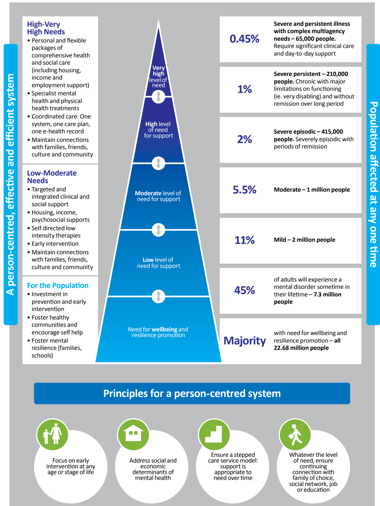
Figure 4: Population-based architecture
